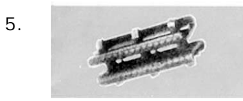
Train Lighting Belt Fastener Walker Type As per RDSO Drg. 3714 (ALT-1)
