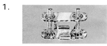
Conveyor Belt Fastener Hawk Type in Size 1, 1.5, 2, 2.5 & 3
