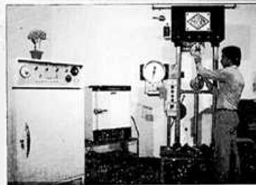
In-house evaluation of Finished Belt on Tensile Testing Machine in the Lab.
